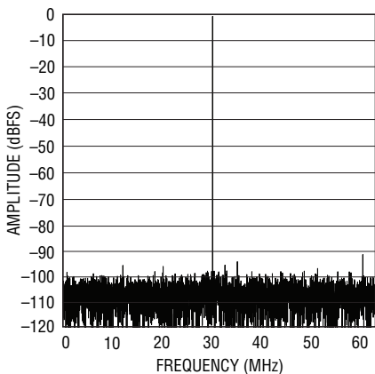
LTC2175-12: 8k Point FFT, f_{IN} = 30\text{MHz} , -1\text{dBFS} , 125Msps
