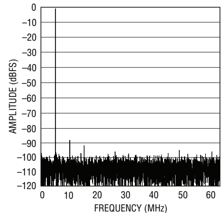
LTC2175-12: 8k Point FFT, f_{IN} = 5\text{MHz} , -1\text{dBFS} , 125Msps
