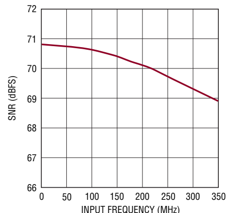
LTC2175-12: SNR vs Input Frequency, -1\text{dB} , 2V Range, 125Msps
