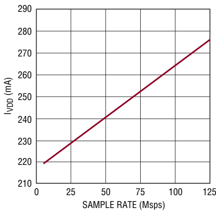
LTC2175-12: I_{VDD} vs Sample Rate, 5MHz Sine Wave Input, -1dB
