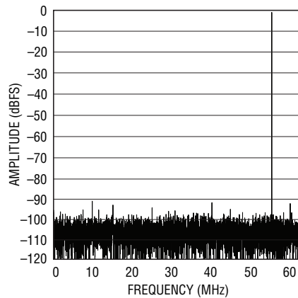
LTC2175-12: 8k Point FFT, f_{IN} = 70\text{MHz} , -1\text{dBFS} , 125Msps
