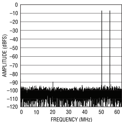
LTC2175-12: 8k Point 2-Tone FFT, f_{IN} = 70\text{MHz} , 75\text{MHz} , -1\text{dBFS} , 125Msps
