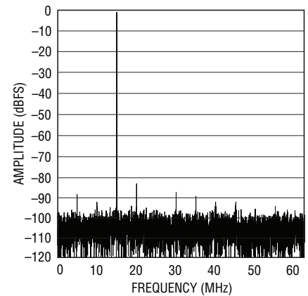
LTC2175-12: 8k Point FFT, f_{IN} = 140\text{MHz} , -1\text{dBFS} , 125Msps
