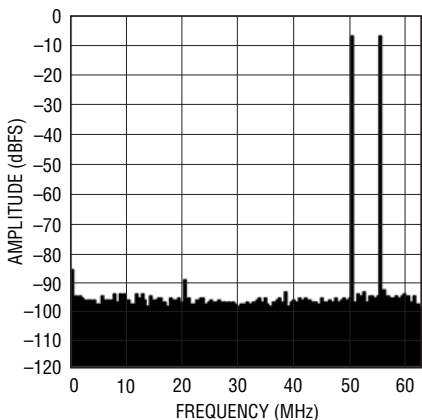
LTC2175-14: 8k Point 2-Tone FFT, f_{IN} = 70\text{MHz}, 75\text{MHz} , -1dBFS, 125Mps
