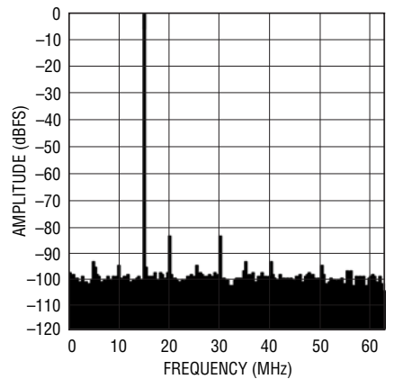
LTC2175-14: 8k Point FFT, f_{IN} = 140\text{MHz} -1dBFS, 125Mps
