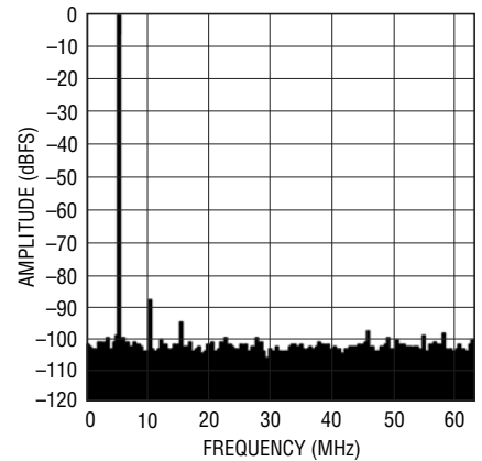
LTC2175-14: 8k Point FFT, f_{IN} = 5\text{MHz} -1dBFS, 125Mps
