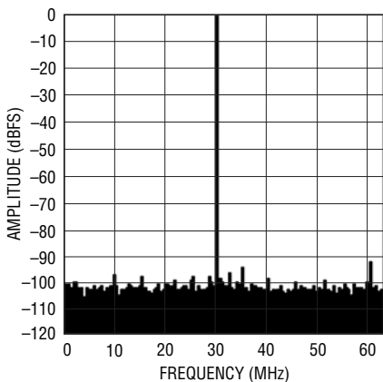
LTC2175-14: 8k Point FFT, f_{IN} = 30\text{MHz} -1dBFS, 125Mps
