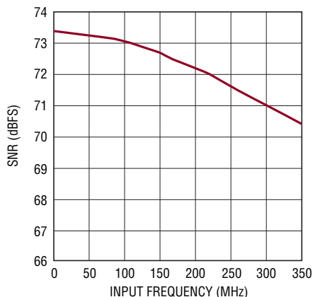
LTC2175-14: SNR vs Input Frequency, -1dB, 2V Range, 125Mps
