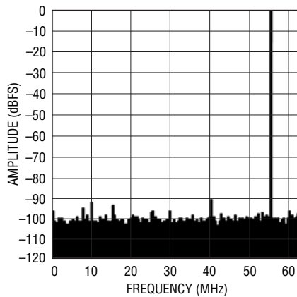
LTC2175-14: 8k Point FFT, f_{IN} = 70\text{MHz} -1dBFS, 125Mps
