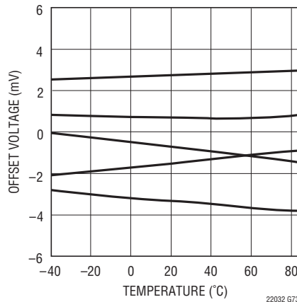
LTC2202: Offset Voltage vs Temperature, 5 Units
