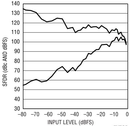
LTC2216 SFDR vs Input Level, f_{IN} = 70.5\text{MHz} , Dither "On"
