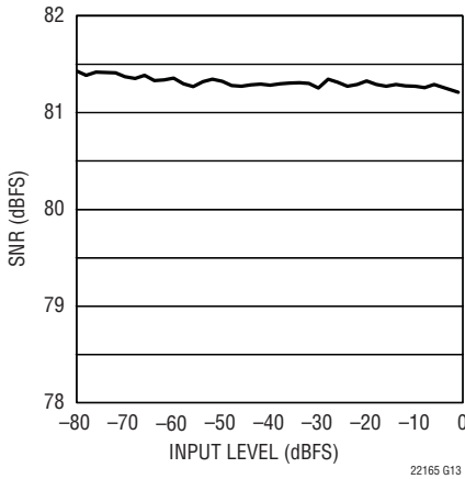
LTC2216 SNR vs Input Level, f IN = 15.2MHz
