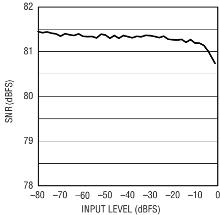
LTC2216 SNR vs Input Level, f_{IN} = 70.5\text{MHz}
