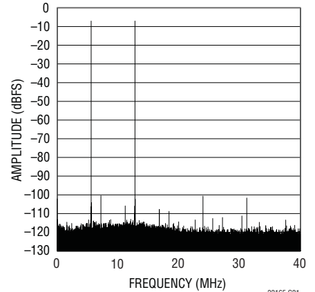
LTC2216 64k Point 2-Tone FFT, f_{IN} = 67.2\text{MHz} and 74.4\text{MHz} , -7\text{dBFS}
