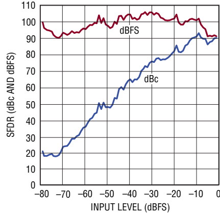
LTC2265-12: SFDR vs Input Level, f_{IN} = 70\text{MHz} , 2V Range, 65Msps
