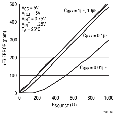
Figure 13. +FS Error vs R_{SOURCE} at \text{REF}^+ or \text{REF}^- (Large C_{REF} )
