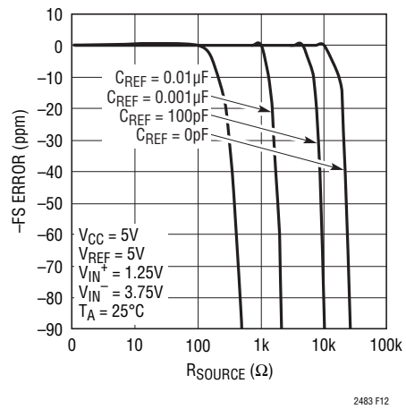
Figure 12. -FS Error vs R_{SOURCE} at \text{REF}^+ or \text{REF}^- (Small C_{REF} )
