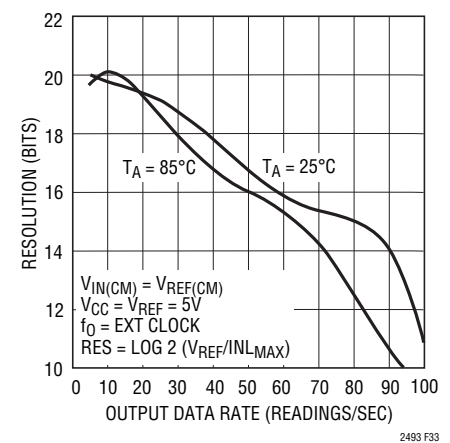
Figure 33. Resolution ( INL_{MAX} \leq 1 LSB) vs Output Data Rate and Temperature
