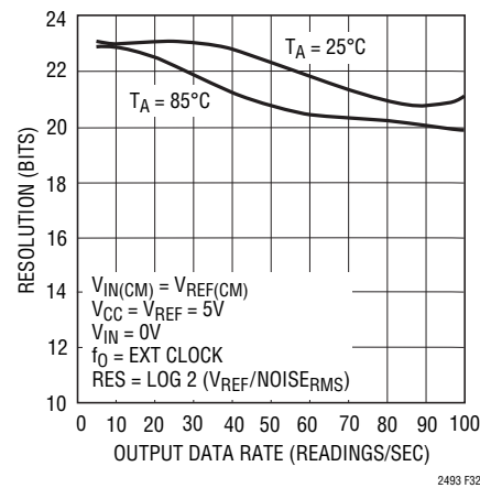
Figure 32. Resolution ( N_{RMS} \leq 1 LSB) vs Output Data Rate and Temperature
