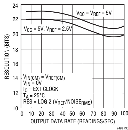
Figure 35. Resolution ( N_{RMS} \leq 1 LSB) vs Output Data Rate and Temperature
