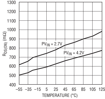
Buck Regulator PMOS R DS(ON) vs Temperature (LTC3559)
