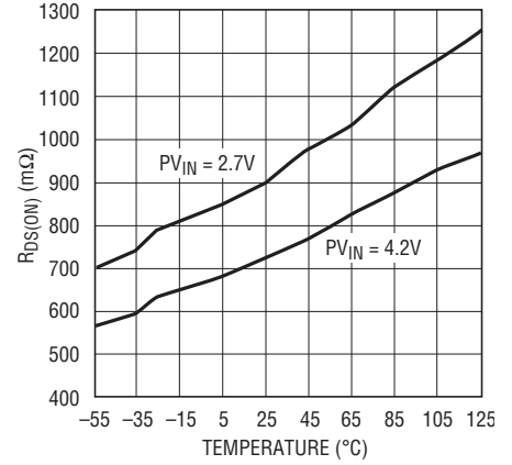
Buck Regulator NMOS R DS(ON) vs Temperature (LTC3559)
