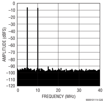
LTM9009-14: 8k Point 2-Tone FFT, f_{IN} = 70\text{MHz} , 75\text{MHz} , -7\text{dBFS} per Tone, 80Msps
