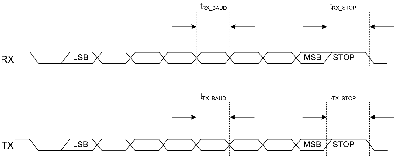
Figure 7 Byte-level Timing
