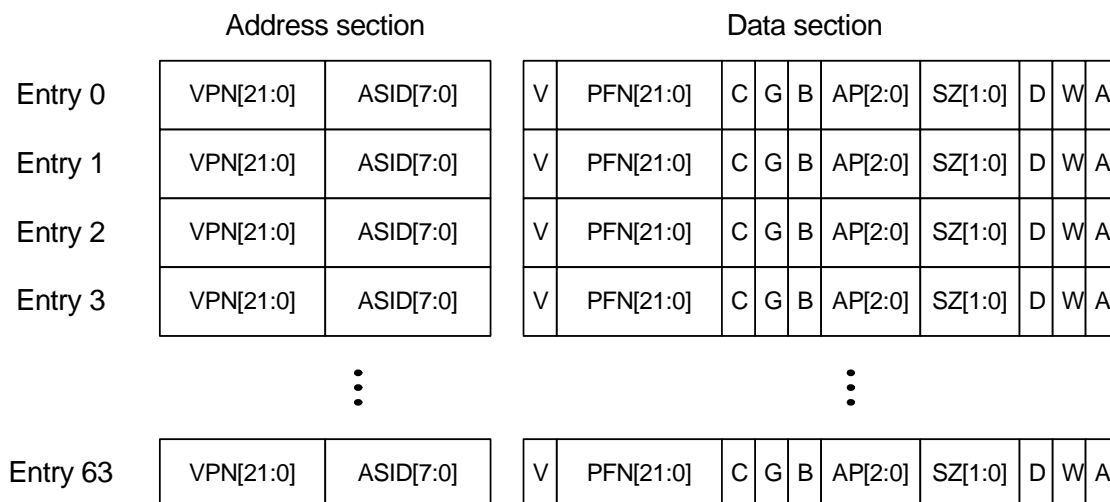
Figure 4-5. TLB organization
