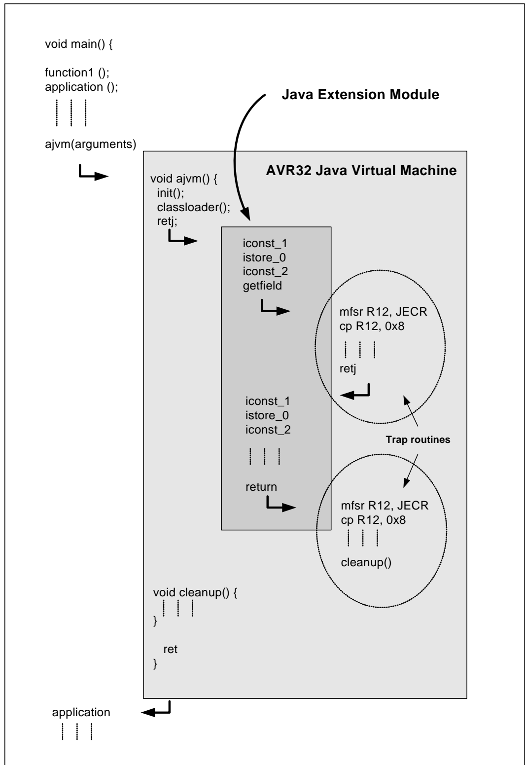
Figure 3-3. Example of running a Java program
