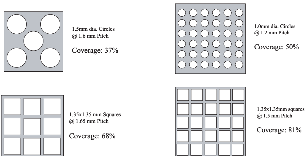
Figure 4-1. Thermal Pad Stencil Designs for 7x7 and 10x10mm MLF Packages
