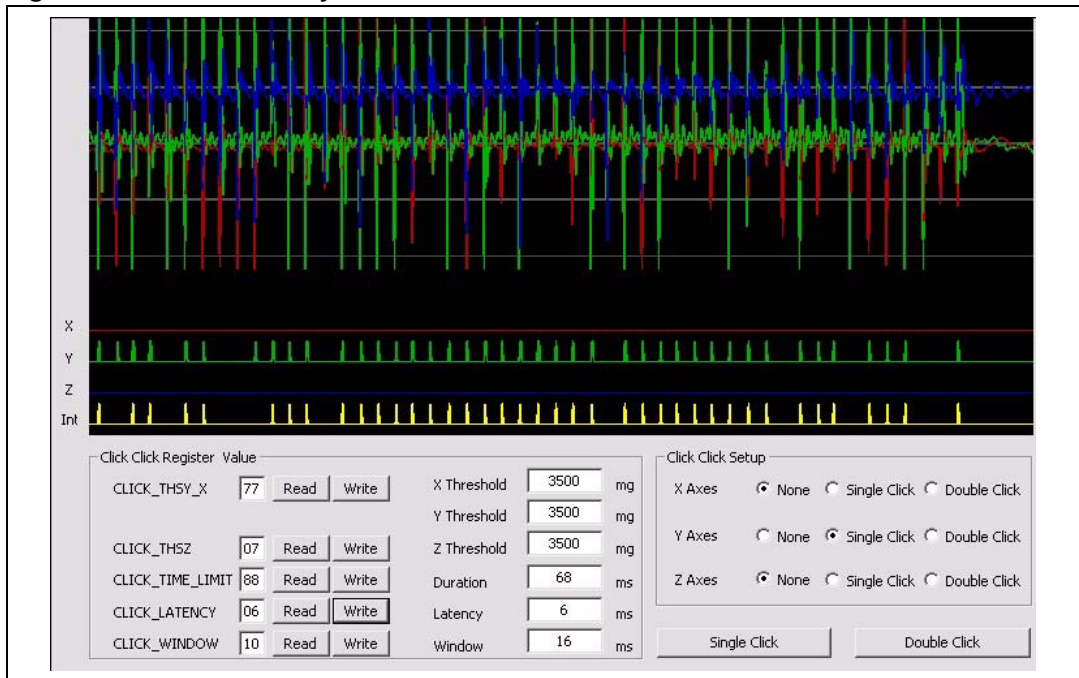
Figure 7. Long Latency
