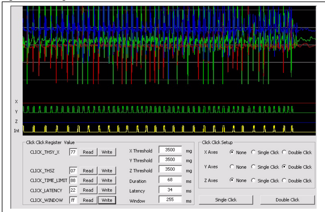
Figure 9. Long Window
