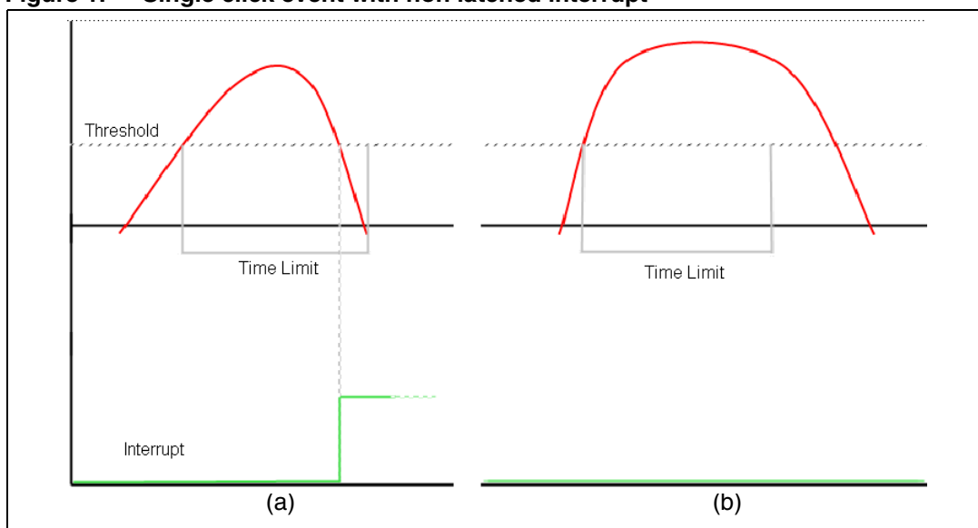
Figure 1. Single click event with non latched interrupt
