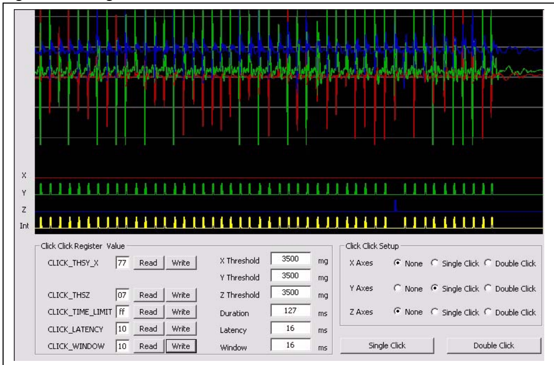
Figure 5. Long TimeLimit
