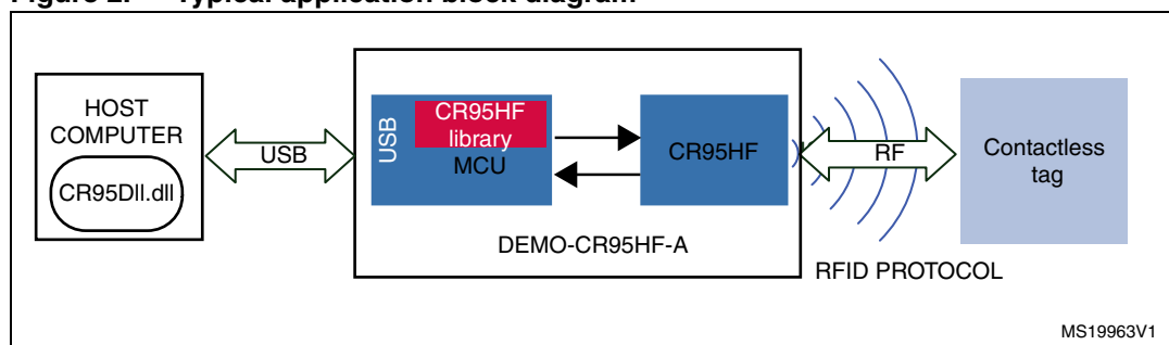
Figure 2. Typical application block diagram
