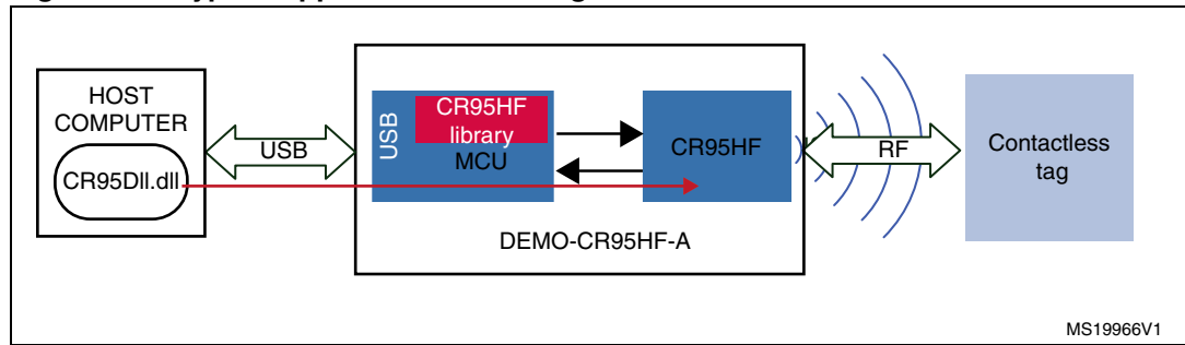
Figure 5. Typical application block diagram
