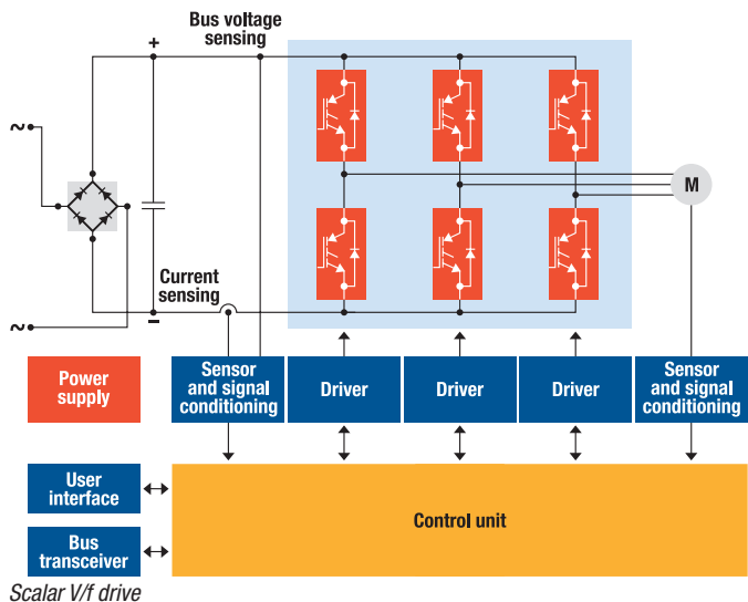
Scalar V/f drive
