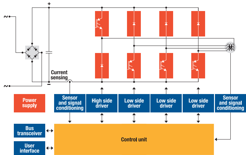
Simplified asymmetrical half-bridge PWM drive
