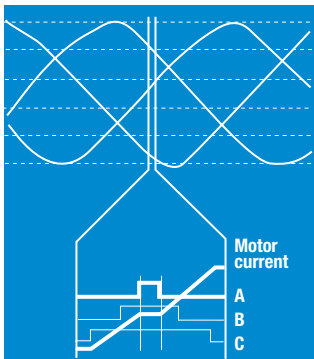
Centered pattern switching
