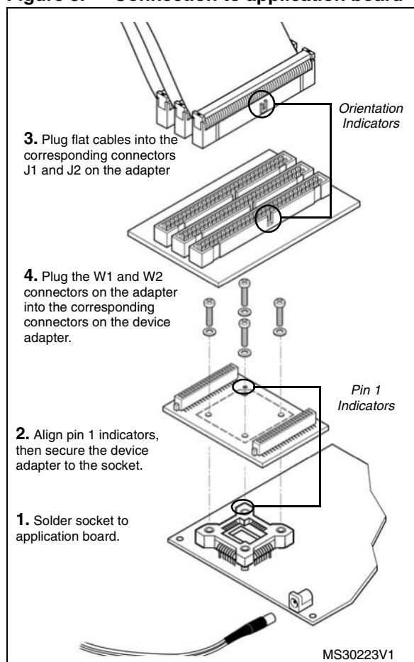
Figure 3. Connection to application board
