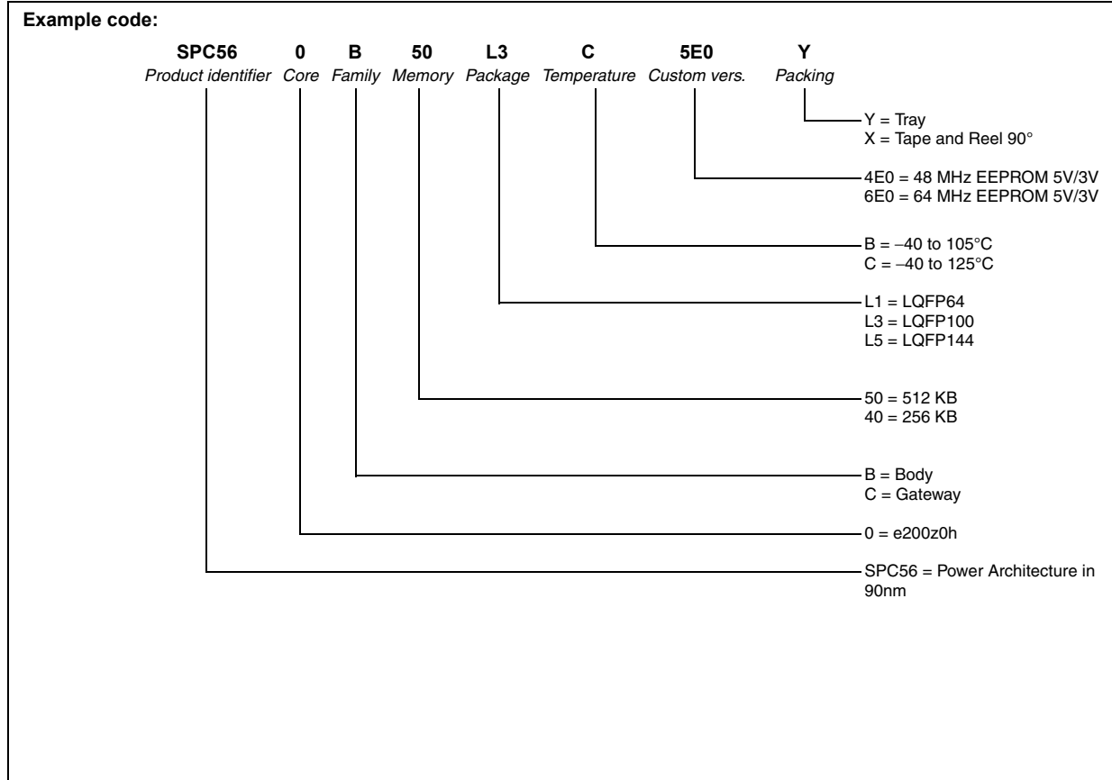
Figure 4. Ordering information scheme
