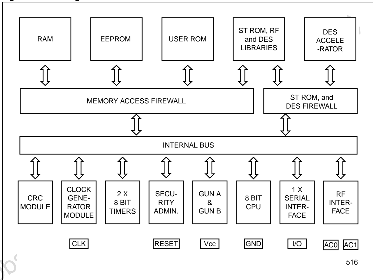
Figure 2. Block Diagram
