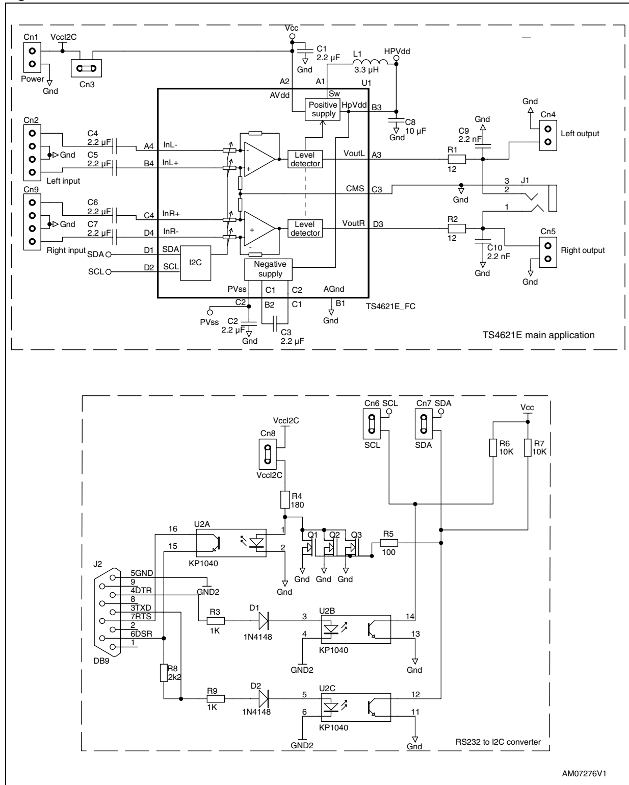
Figure 1. Circuit schematics
