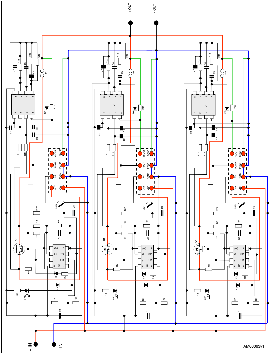
Figure 2. Motherboard circuit schematic
