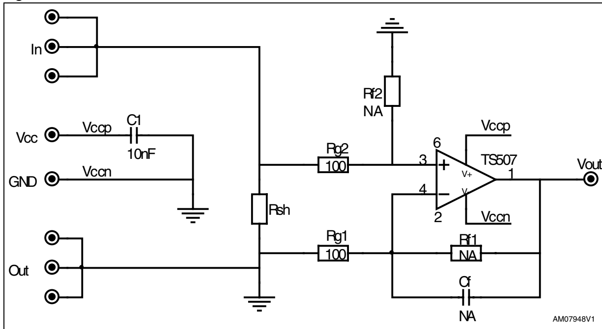
Figure 1. Internal schematic
