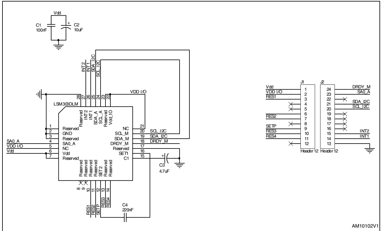
Figure 1. Schematic circuit
