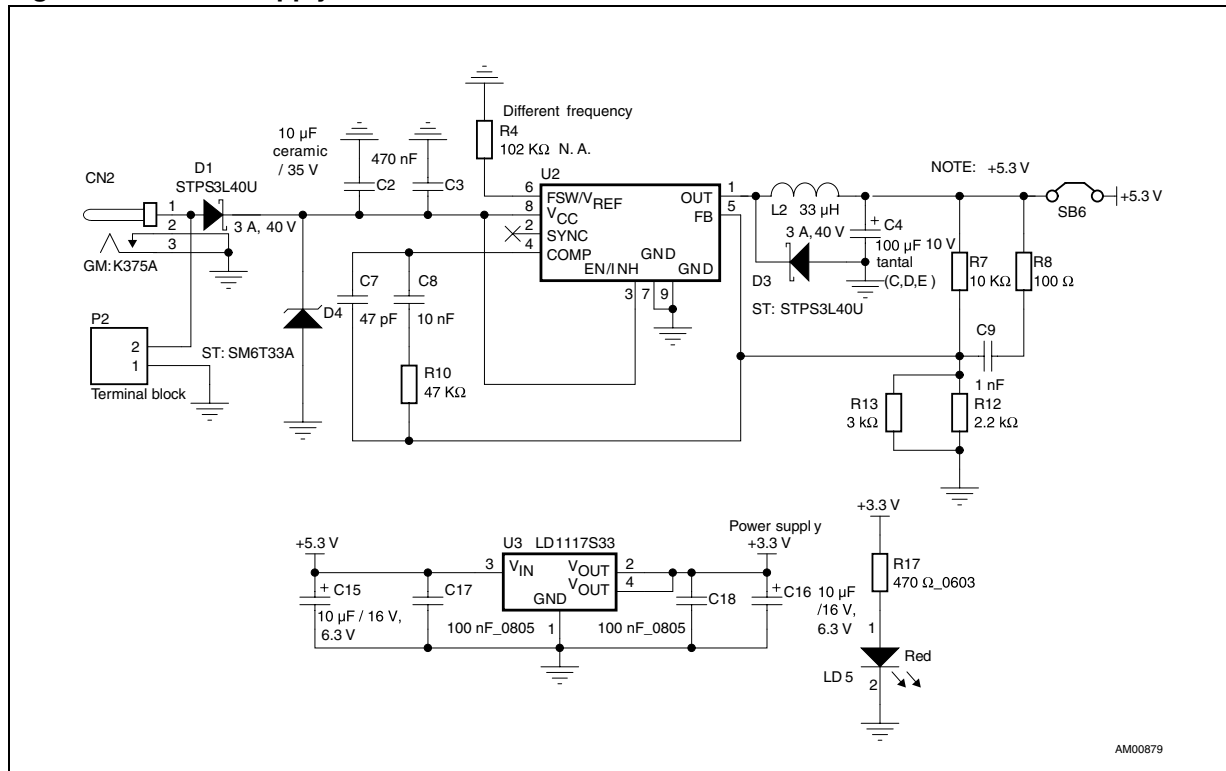
Figure 1. Power supply
