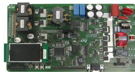
System evaluation board (STEVAL-ISV003V1)
