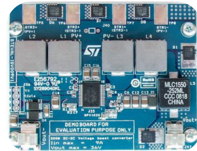
System evaluation board (STEV009V1)
