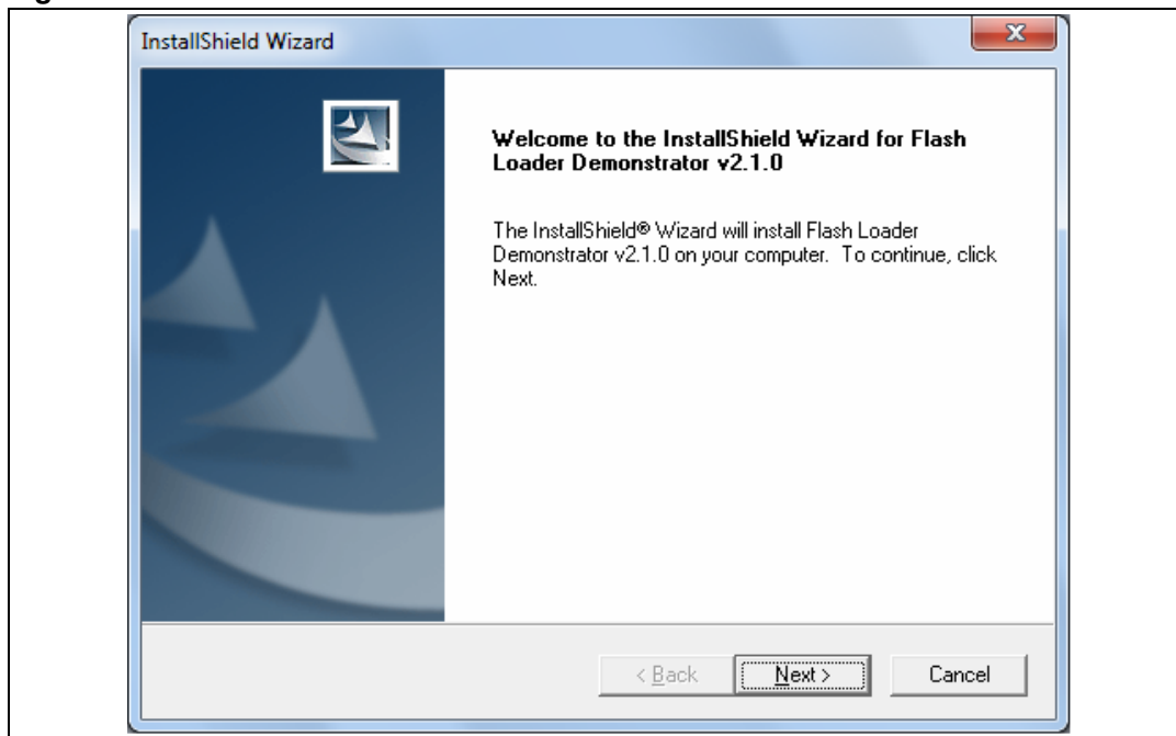
Figure 3. InstallShield Wizard
