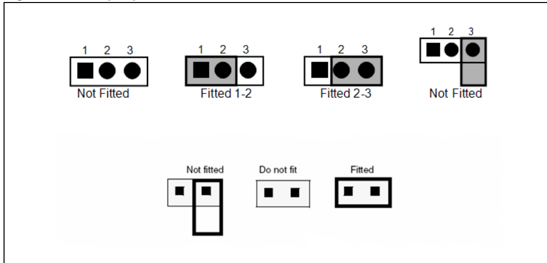
Figure 2. Jumper position
