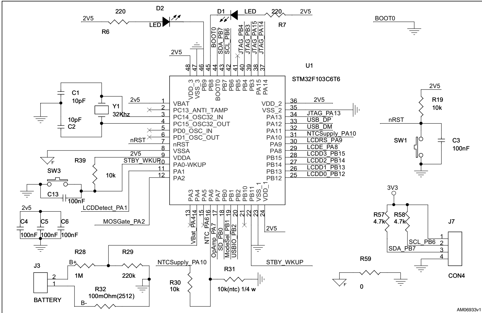
Figure 7. Microcontroller section
