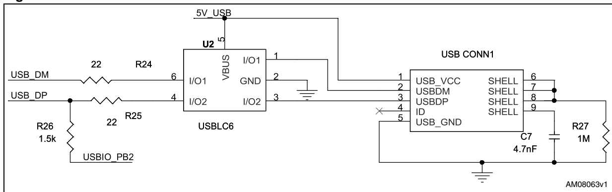
Figure 10. USB section
