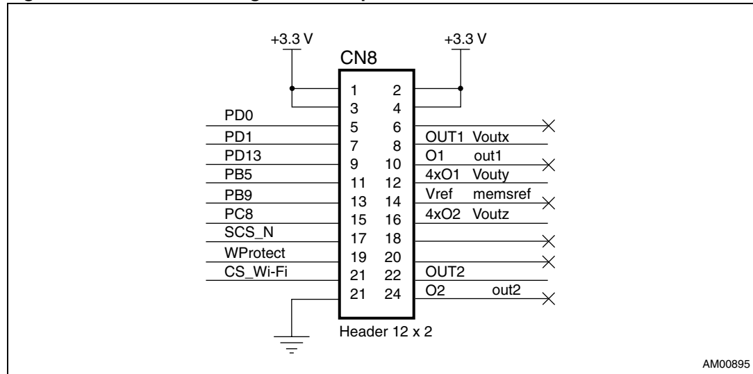
Figure 10. GPIO and analog connector pinout
