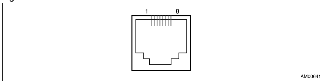
Figure 12. Ethernet RJ45 connectors CN5 - front view
