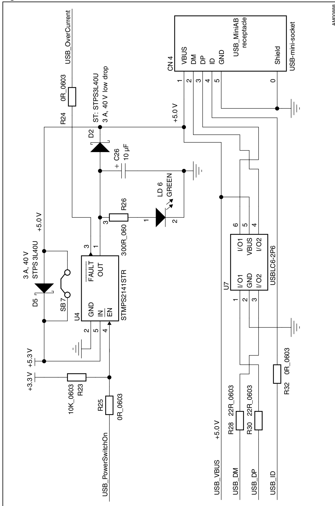
Figure 21. USB-OTG
