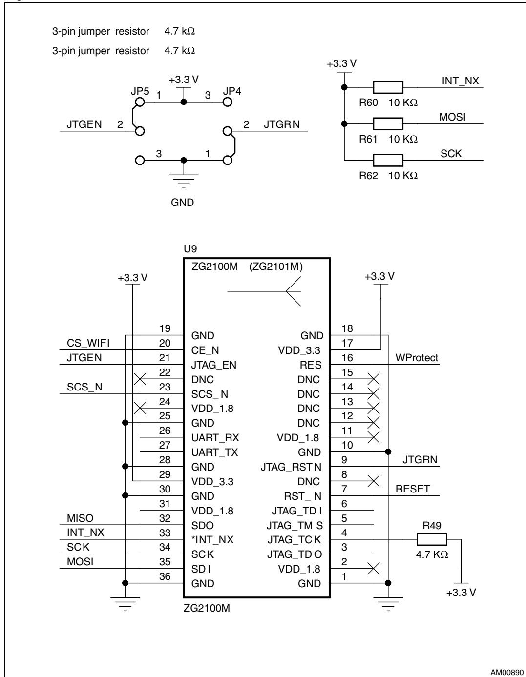
Figure 23. Wi-Fi module-2
