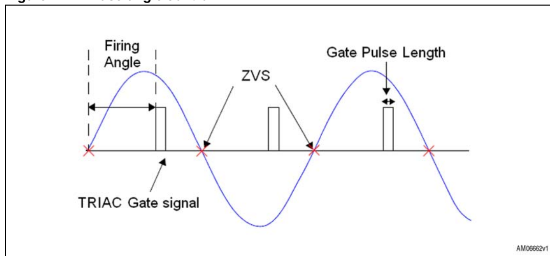
Figure 4. Phase-angle control
