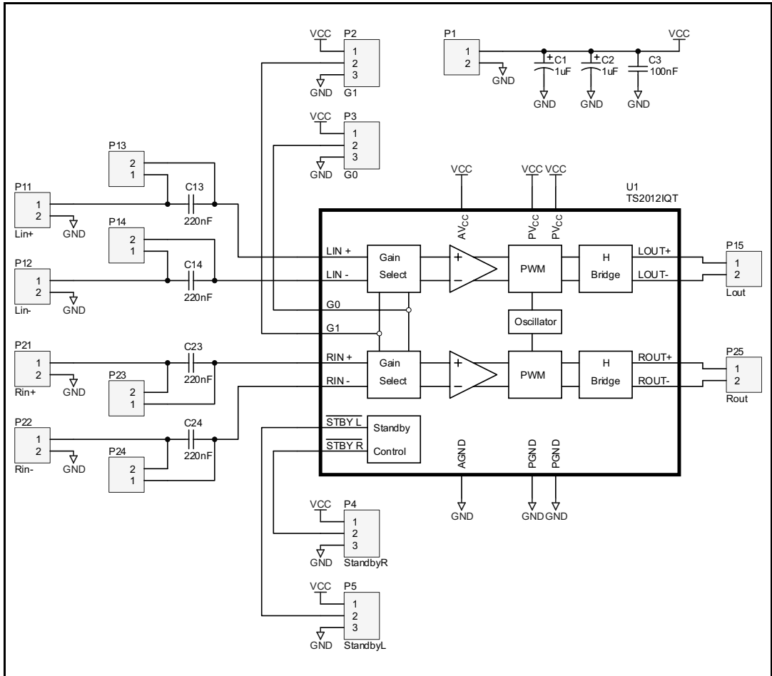
Schematic diagram
