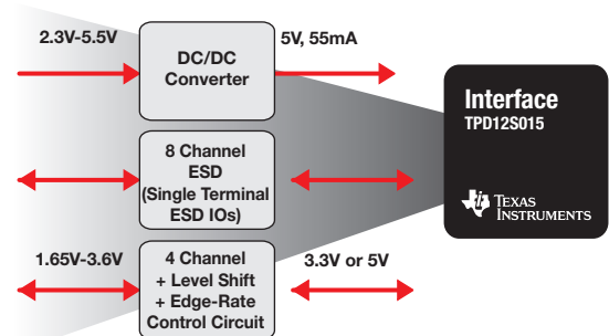
TPD12S015 illustration
