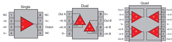
OPA1611/1602/1641 pin configurations
