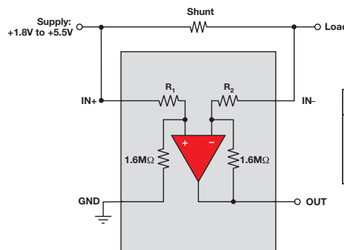
INA216 functional block diagram
