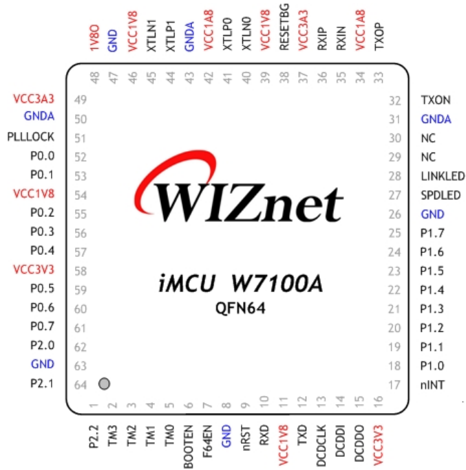
Fig 2. W7100A 64pin QFN package
