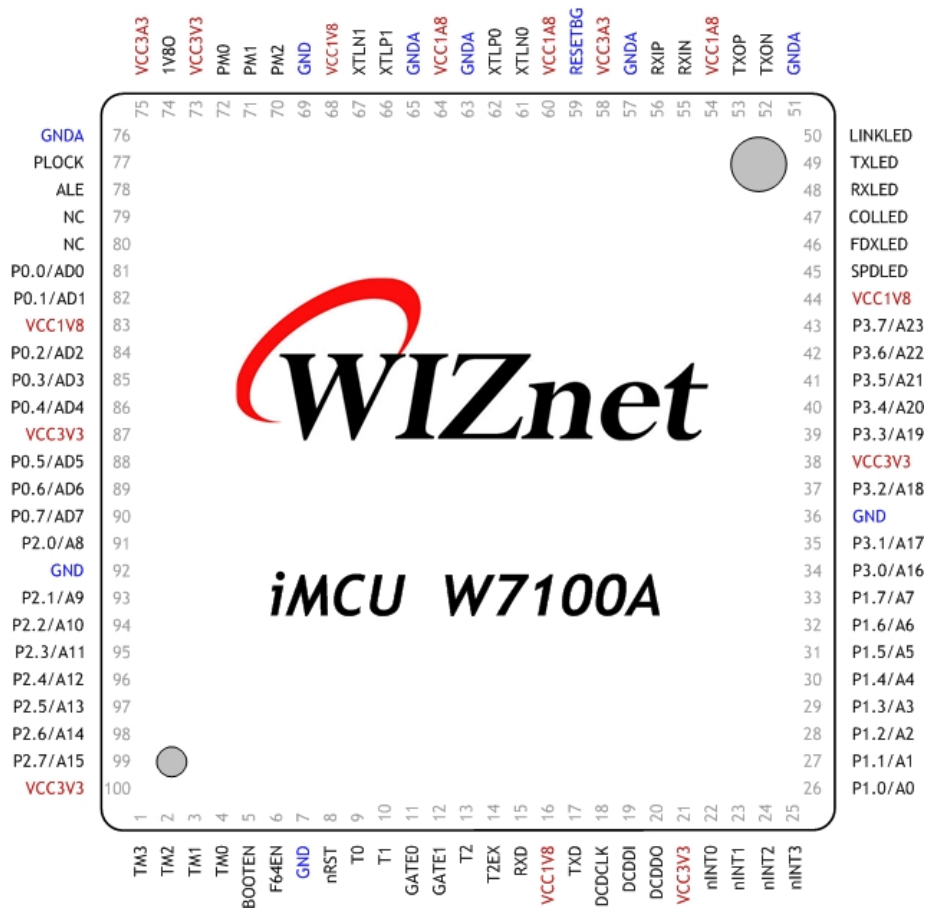
Fig 1. W7100A 100pin LQFP package
