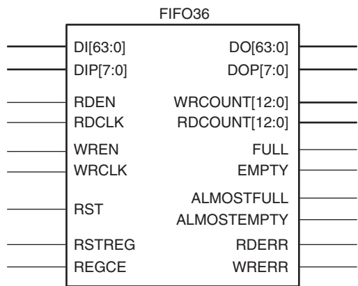
Figure 2-3: FIFO36
