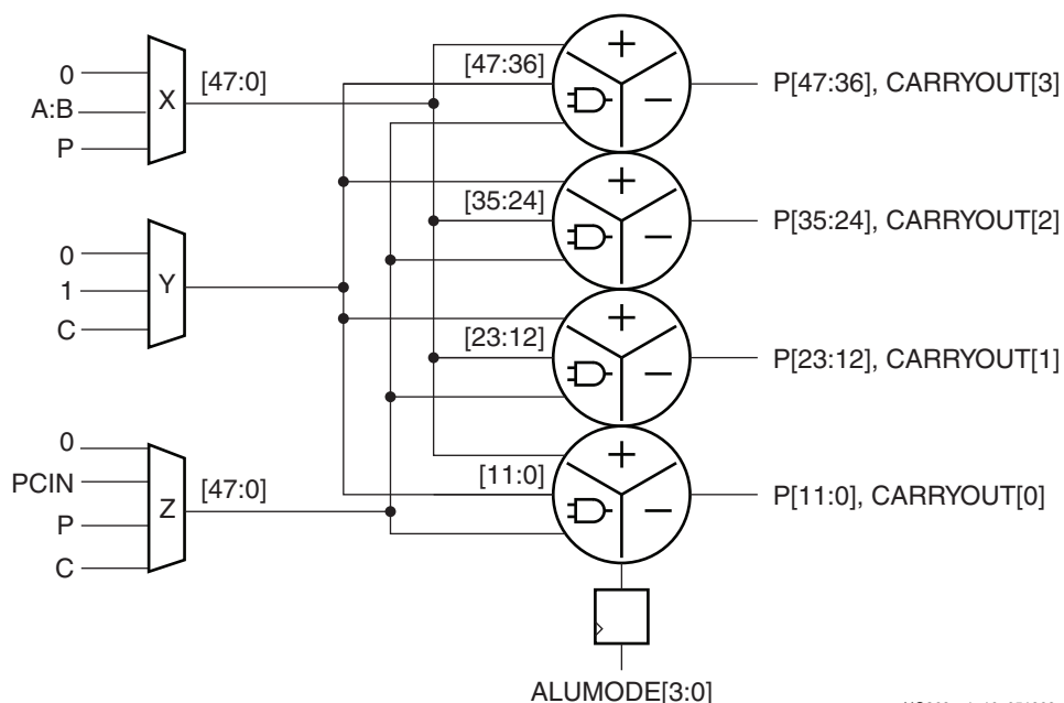
Figure 2-16: Four 12-Bit SIMD Adder Configuration
