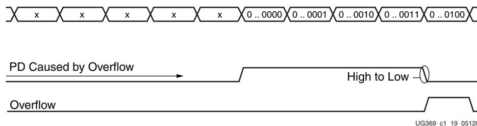
Figure 2-19: Overflow Condition in the Pattern Detector
