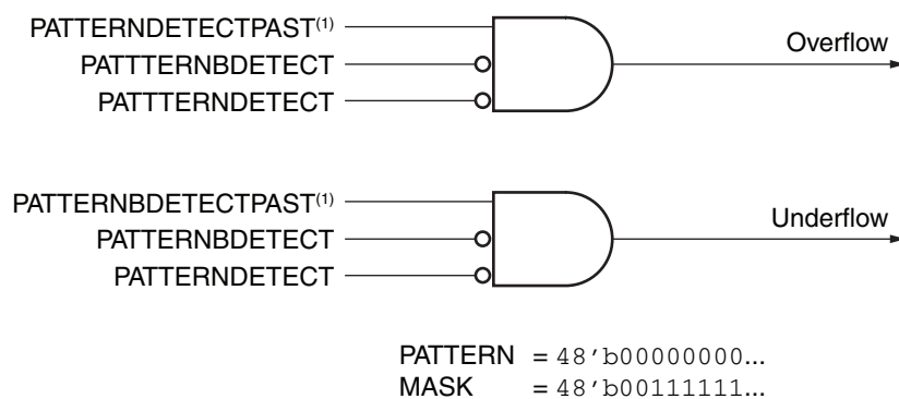
Figure 2-18: Overflow/Underflow Logic in Pattern Detect
