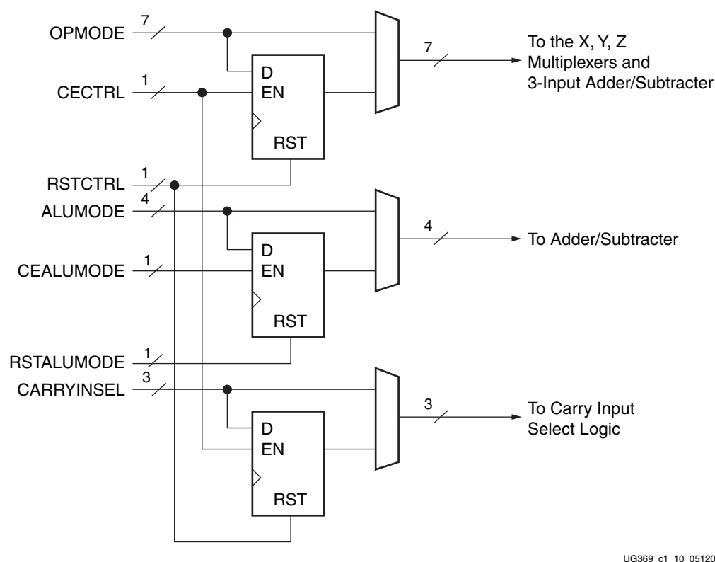
Figure 2-10: OPMODE, ALUMODE, and CARRYINSEL Port Logic
