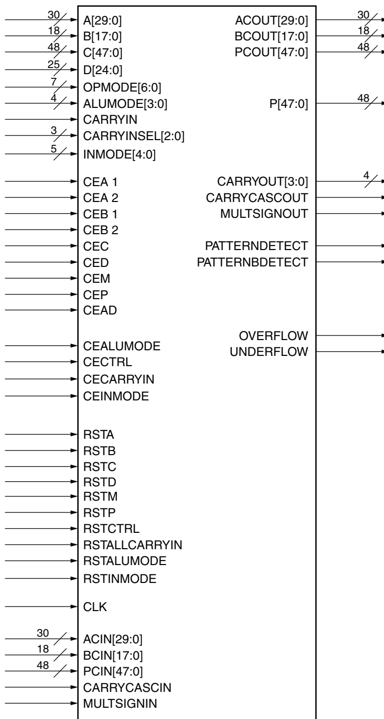
Figure 2-4: DSP48E1 Slice Primitive
