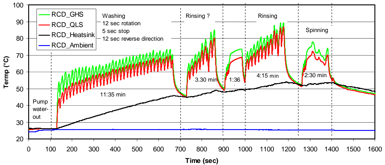
Case Temperature Profile during "20min" cycle Infineon RCD in I-pak IKU06N60R
