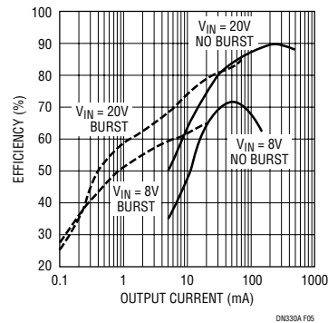
Figure 5. 8V-60V to 12V Conversion Efficiency
