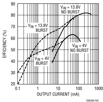
Figure 3. 4V-60V to 5V Conversion Efficiency
