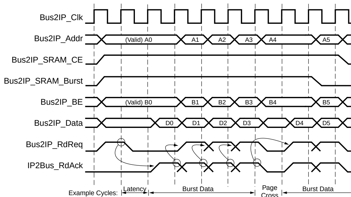
Figure 6-18: IPIF Slave SRAM Module Read Burst Transaction
