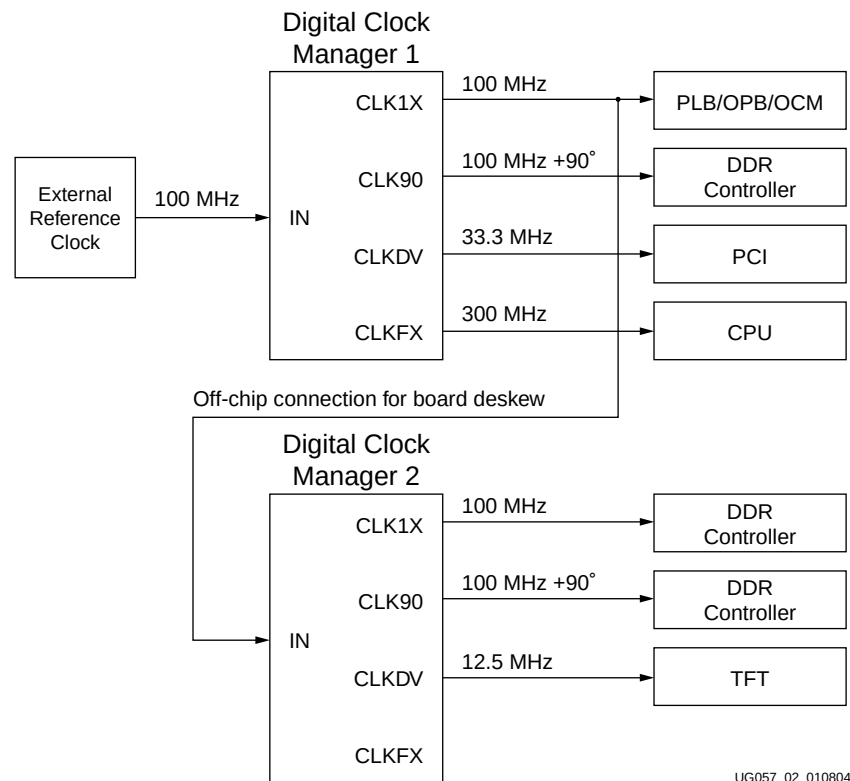
Figure 2-2: Clock Generation
