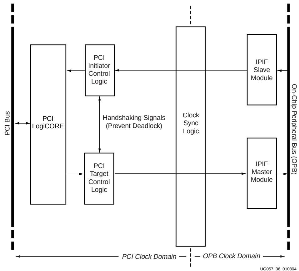
Figure 7-1: OPB to PCI Bridge
