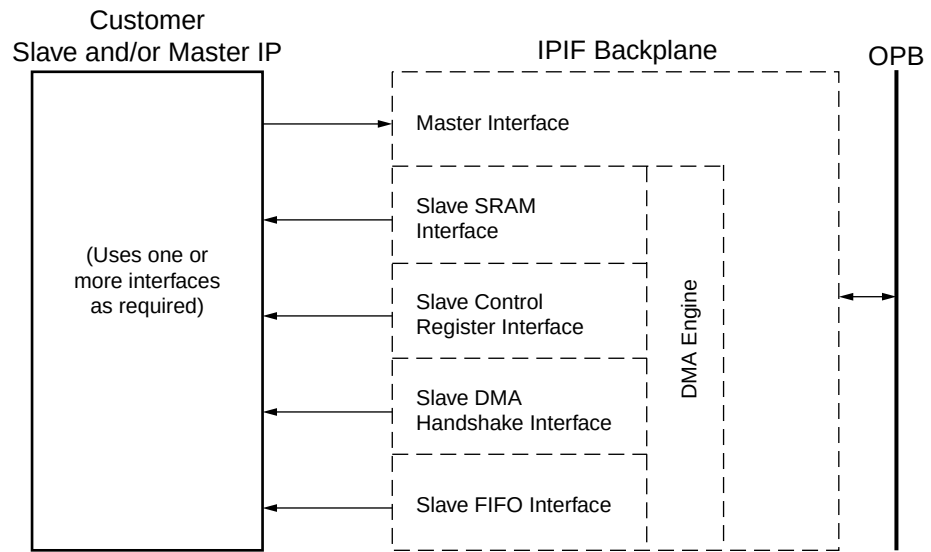
Figure 6-2: General Model of the IPIF Backplane
