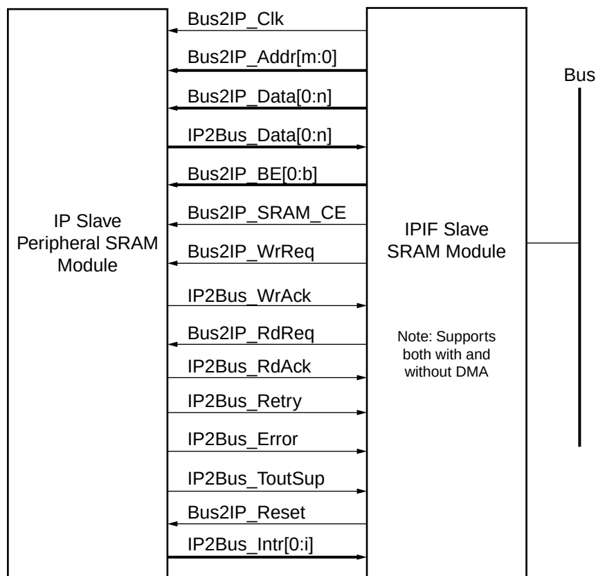
Figure 6-14: Slave IP Module SRAM Protocol Block Diagram
