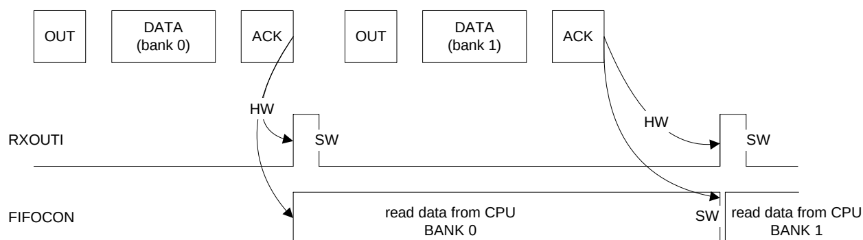
Figure 25-24. Example of an OUT Endpoint with 2 Data Banks
