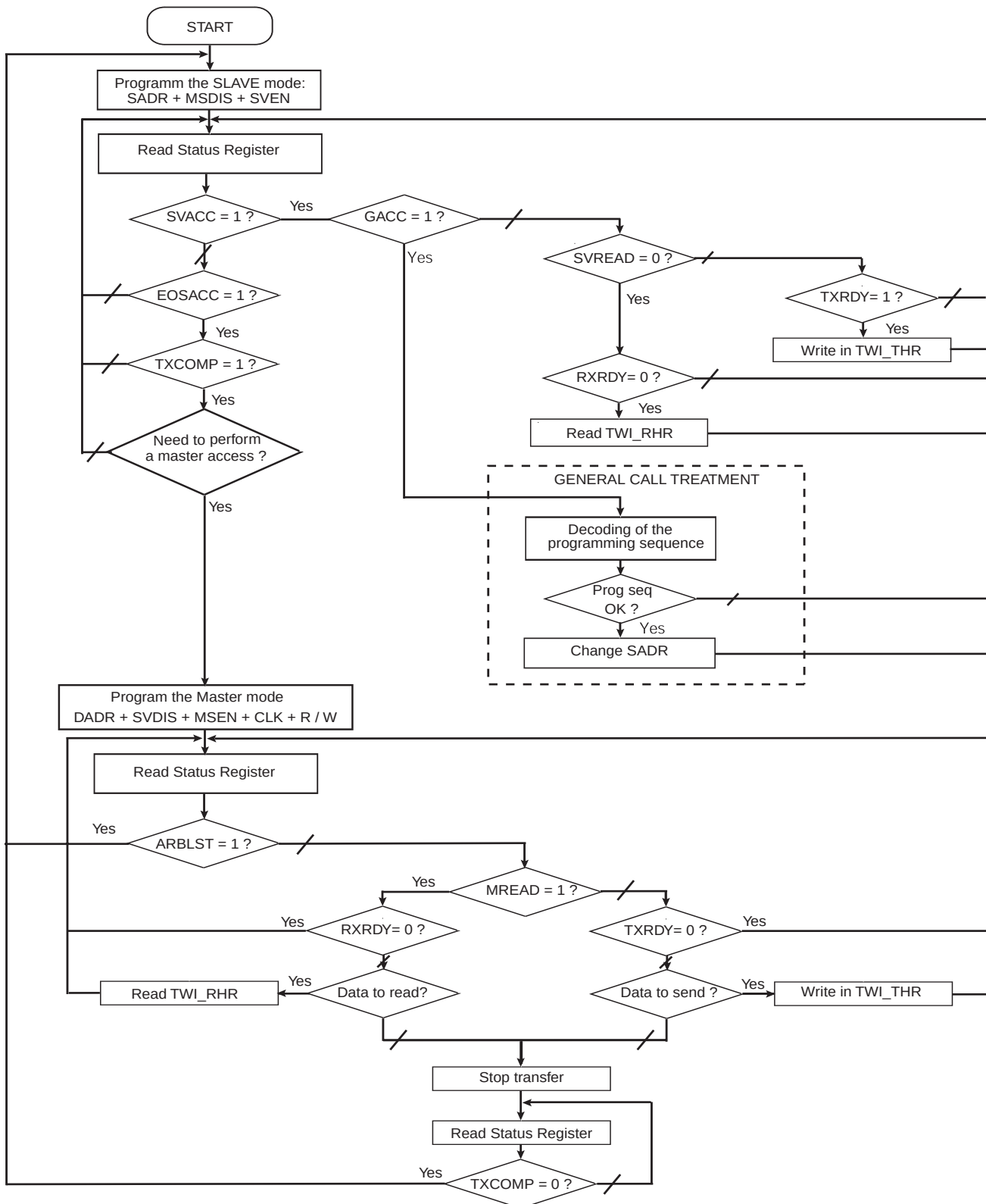
Figure 22-21. Multi-master Flowchart
