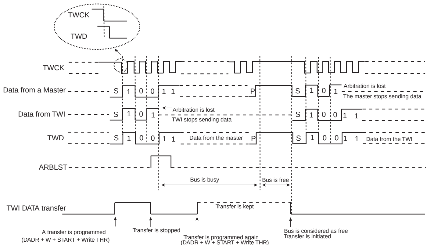
Figure 22-20. Arbitration Cases
