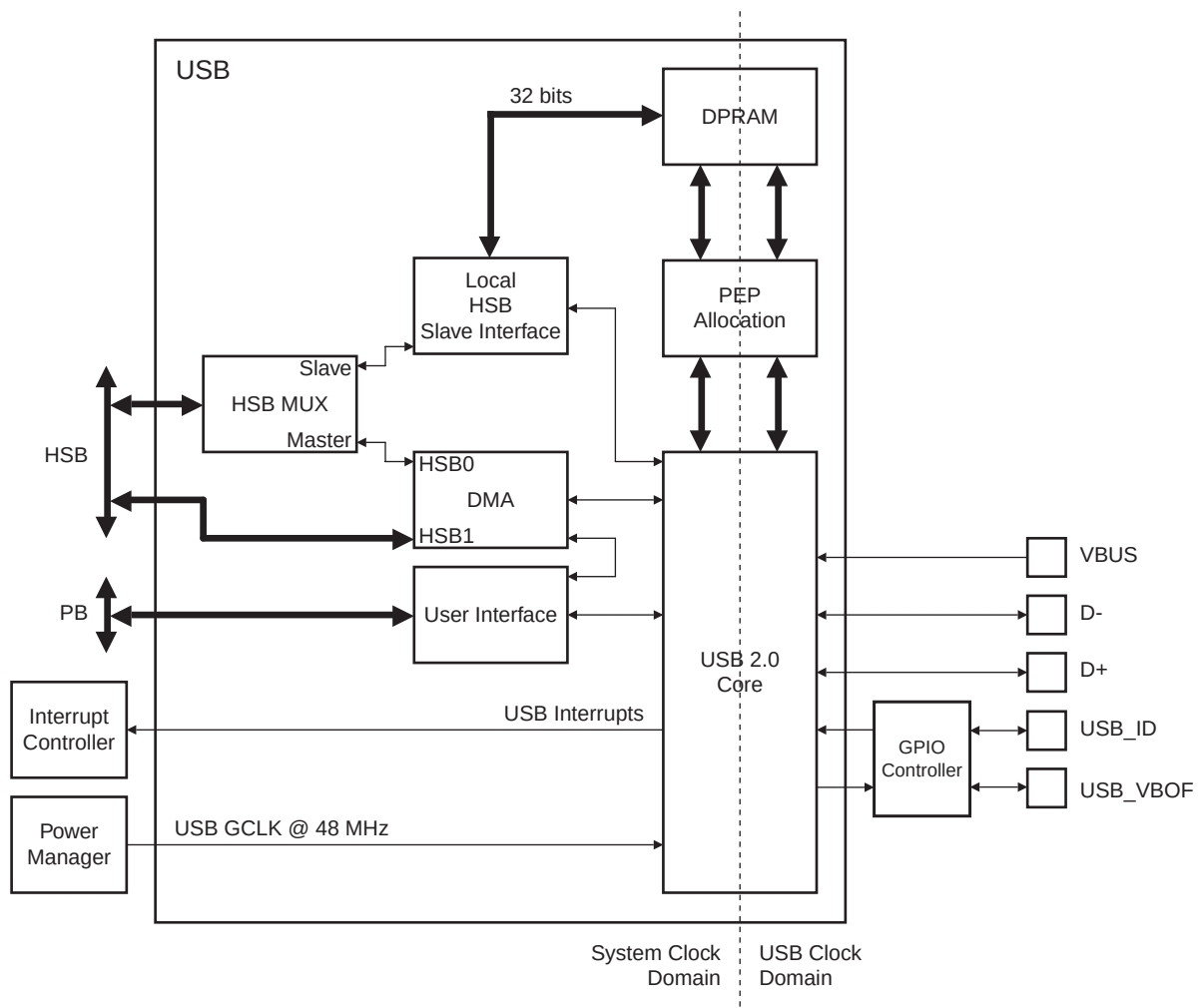
Figure 25-1. Block Diagram
