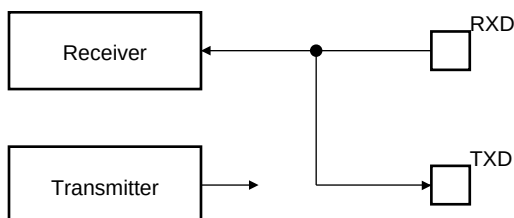
Figure 24-41. Automatic Echo Mode Configuration
