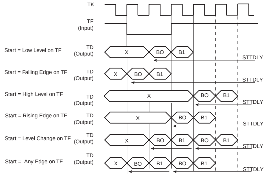
Figure 23-10. Transmit Start Mode
