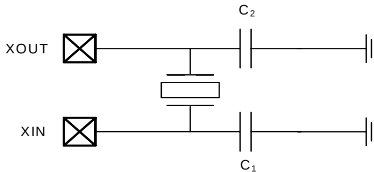
Figure 12-2. Oscillator connections
