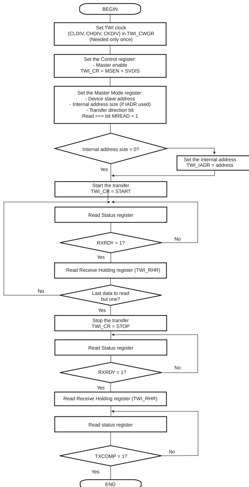
Figure 22-18. TWI Read Operation with Multiple Data Bytes with or without Internal Address
