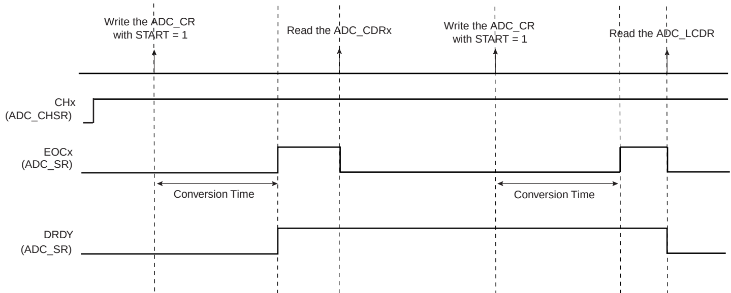
Figure 28-2. EOCx and DRDY Flag Behavior
