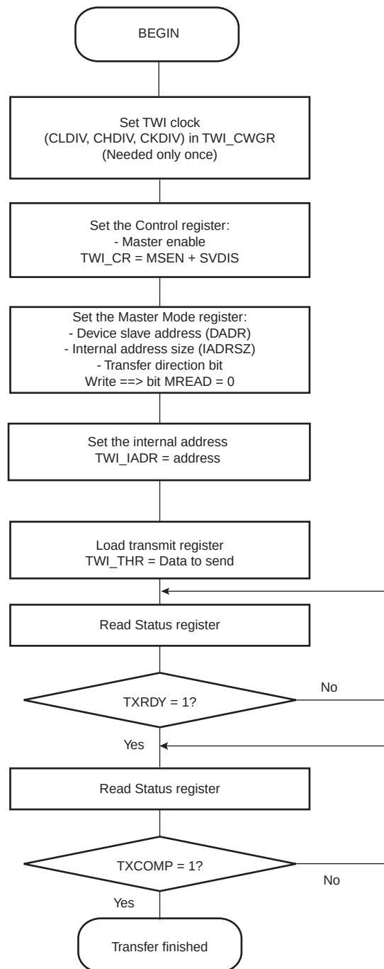
Figure 22-14. TWI Write Operation with Single Data Byte and Internal Address
