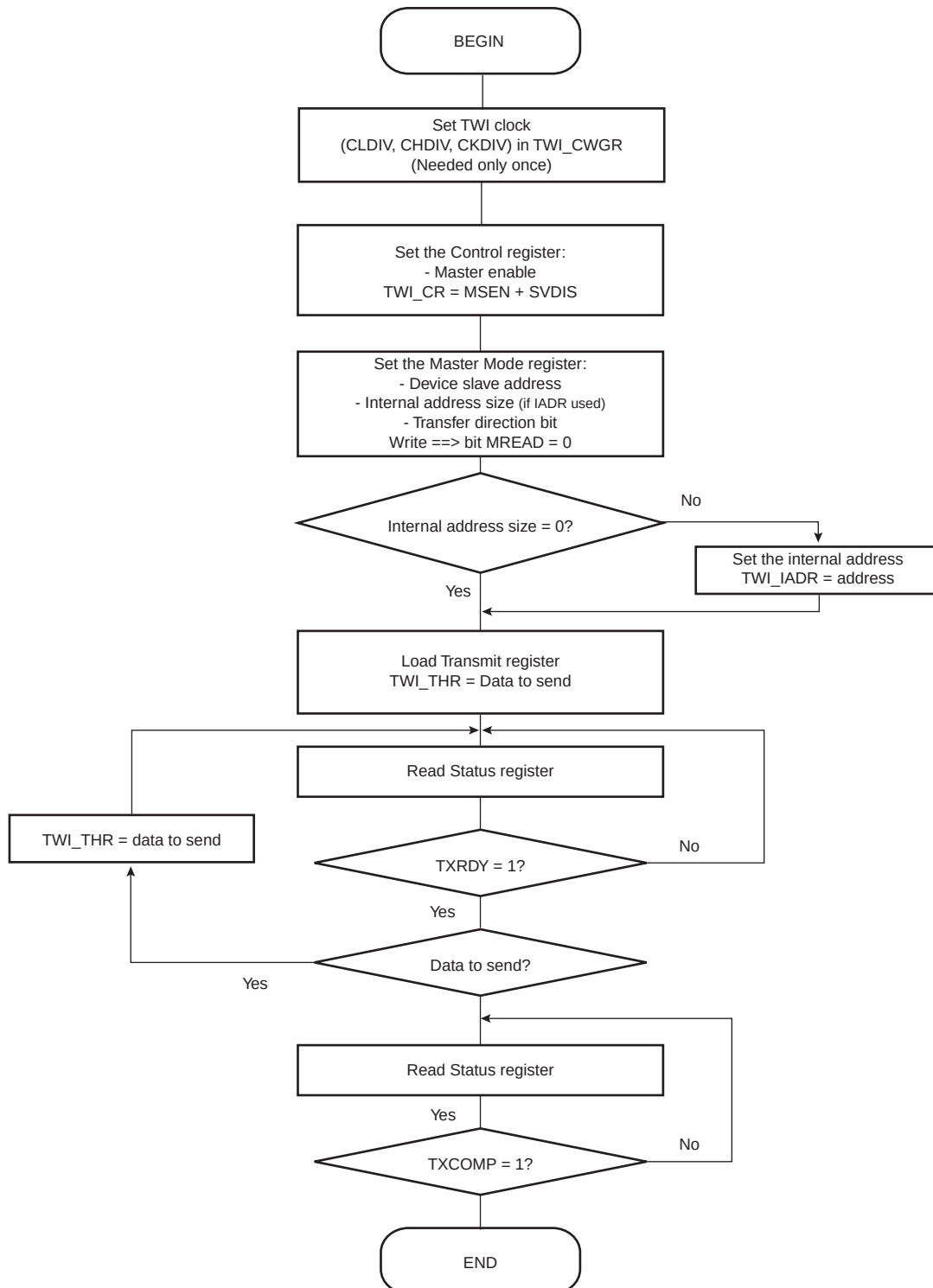
Figure 22-15. TWI Write Operation with Multiple Data Bytes with or without Internal Address
