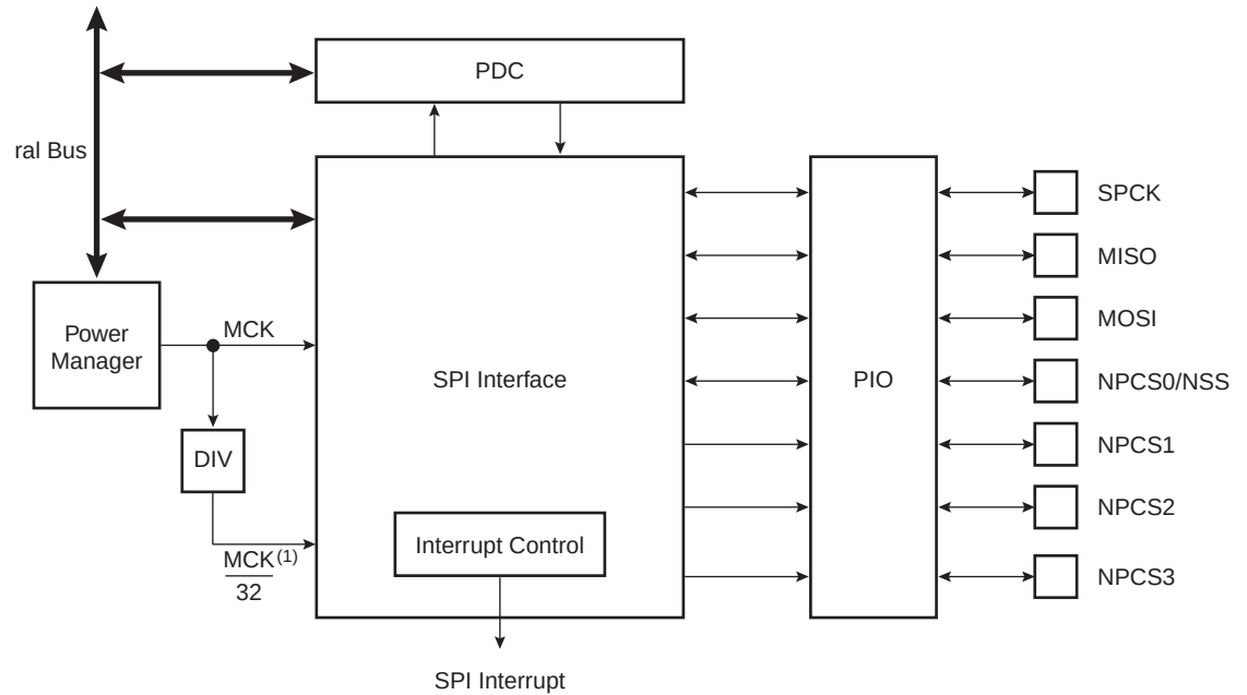
Figure 21-1. Block Diagram
