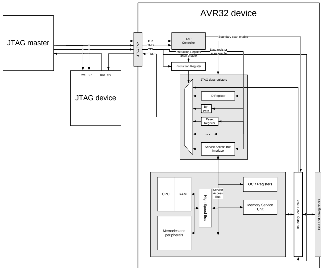
Figure 30-1. JTAG and Boundary Scan access
