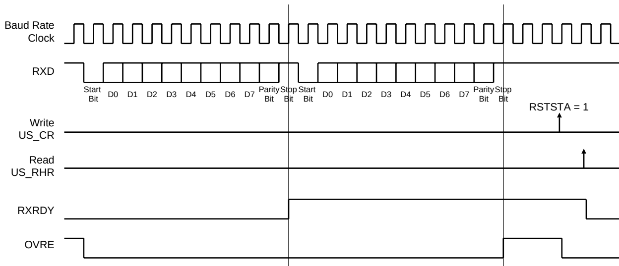
Figure 24-21. Receiver Status
