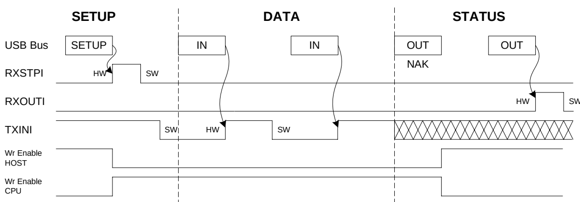
Figure 25-19. Control Read
