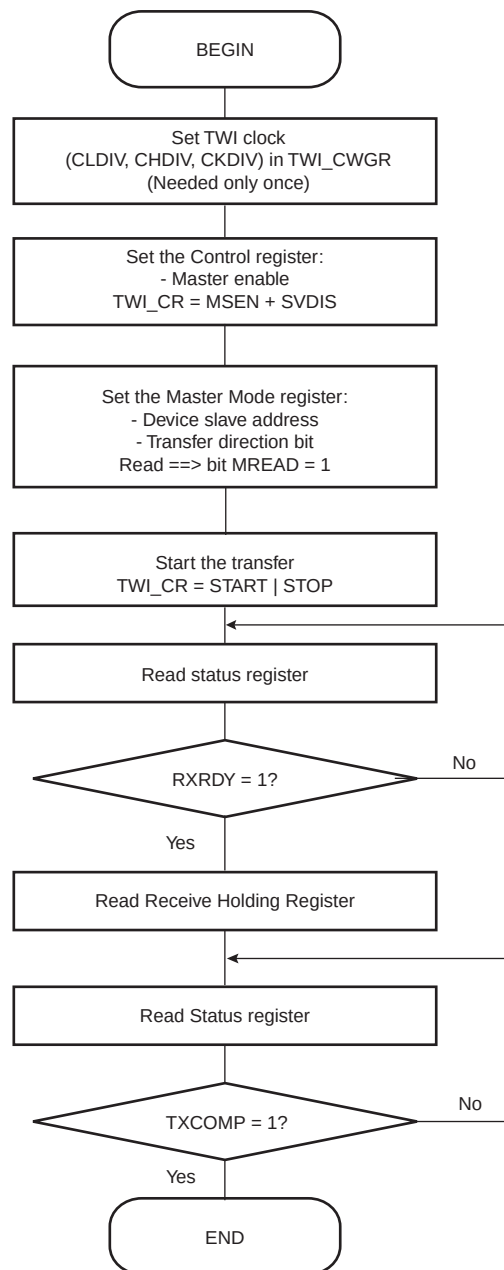
Figure 22-16. TWI Read Operation with Single Data Byte without Internal Address
