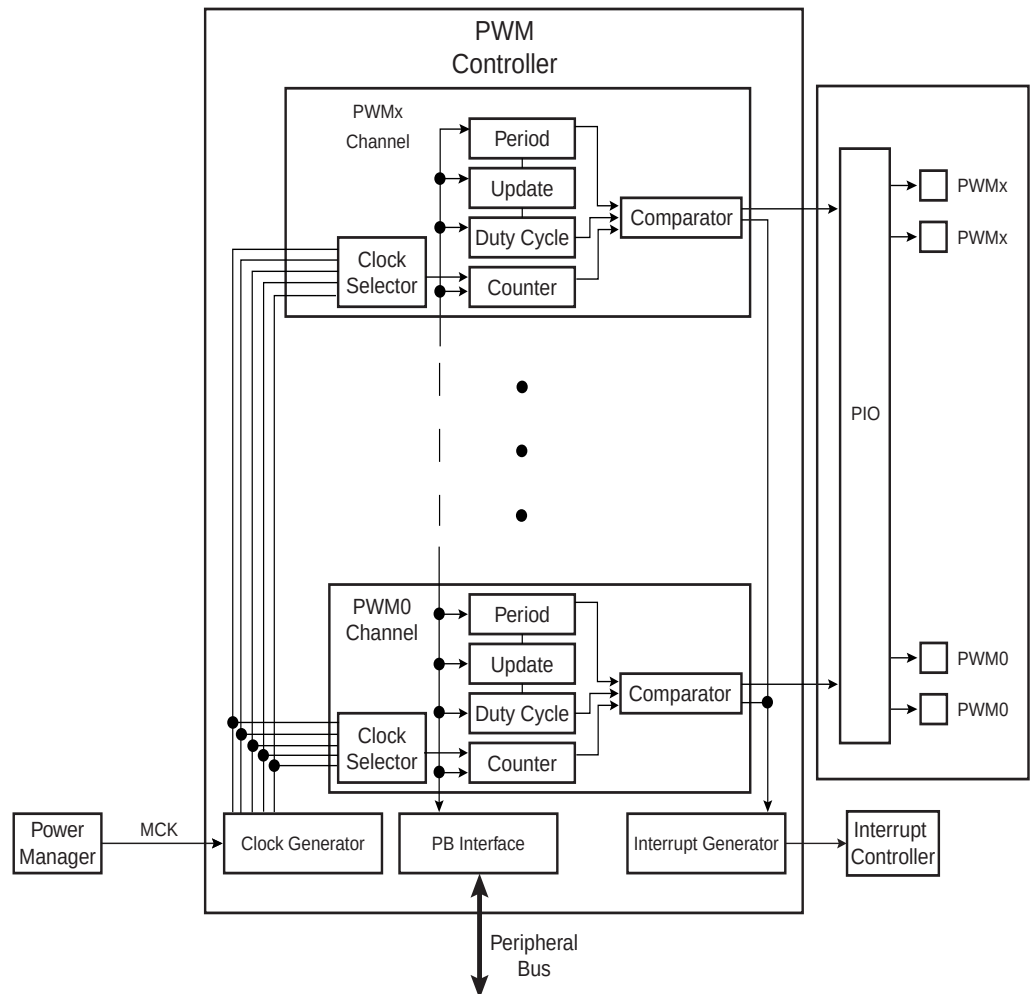
Figure 27-1. Pulse Width Modulation Controller Block Diagram
