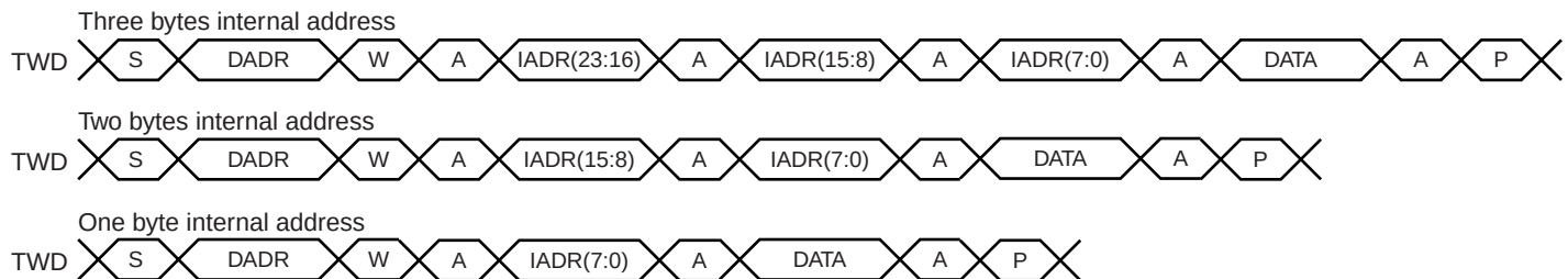
Figure 22-11. Master Write with One, Two or Three Bytes Internal Address and One Data Byte
