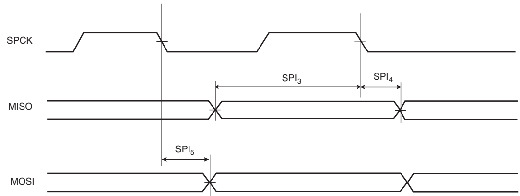
Figure 32-5. SPI Master mode with (CPOL=0 and NCPHA=1) or (CPOL=1 and NCPHA=0)
