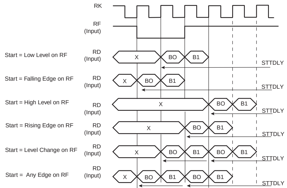
Figure 23-11. Receive Pulse/Edge Start Modes
