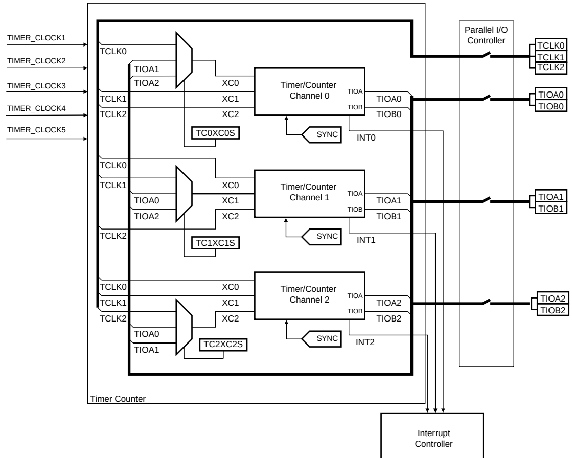
Figure 26-1. Timer Counter Block Diagram
