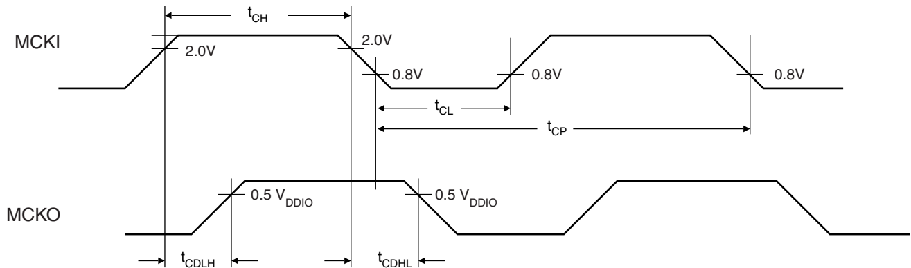
Figure 19-1. Clock Waveform
