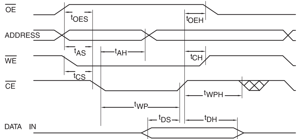
Figure 20-15. CE Controlled
