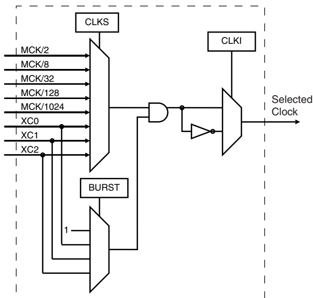
Figure 18-2. Clock Selection
