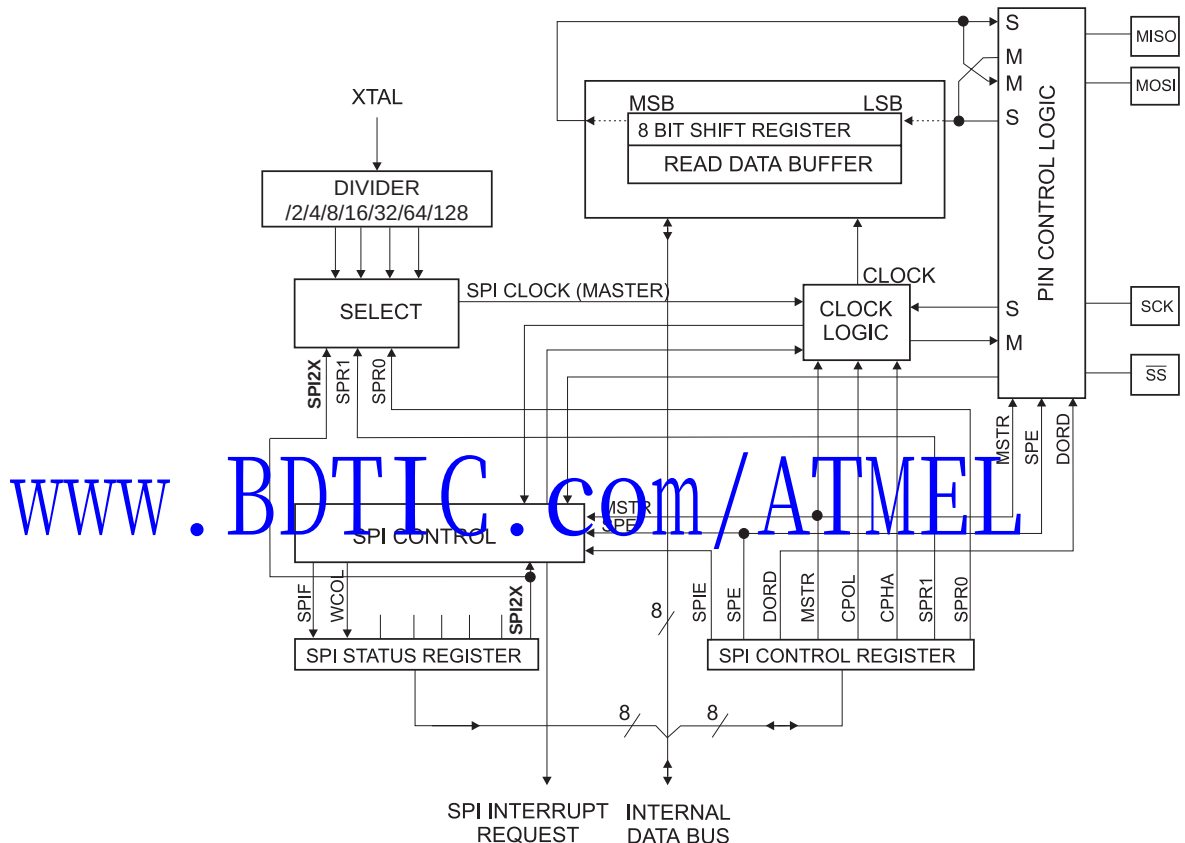
Figure 65. SPI 方框图 (1)
