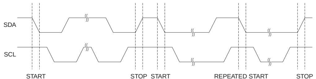
Figure 78. START、REPEATED START 与 STOP 状态
