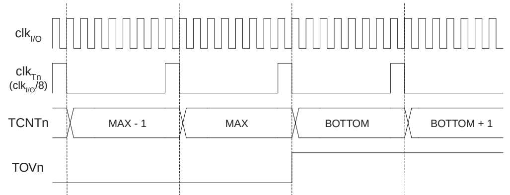
Figure 35. T/C 时序图, 预分频器为 f_{\text{clk\_I/O}}/8
