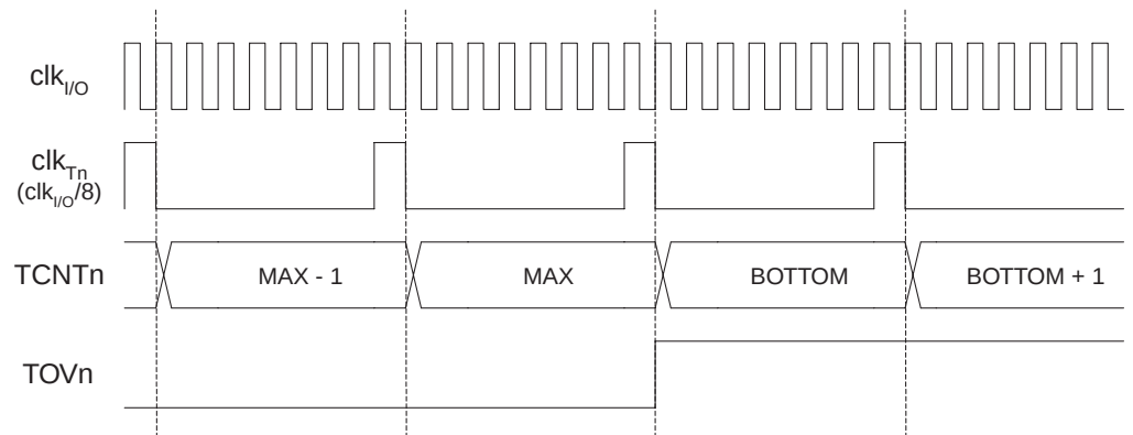
Figure 61. T/C 时序图, 预分频器为 f_{\text{clk}_{I/O}}/8
