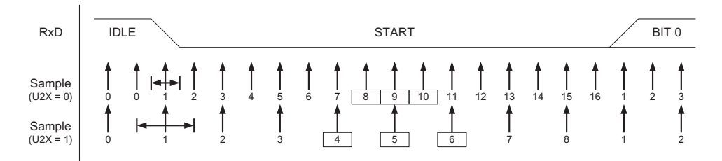
Figure 73. 起始位采样
