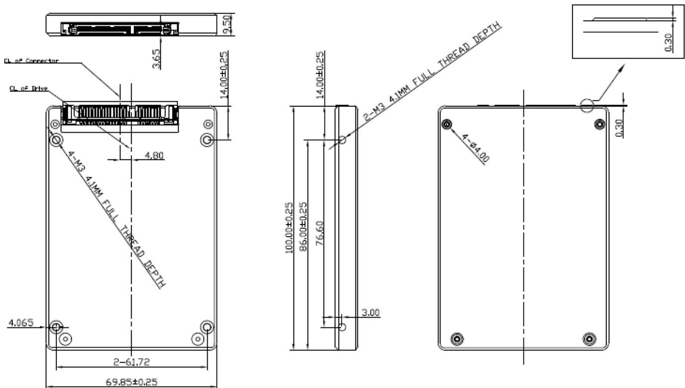
Figure 2-1. Physical dimension
