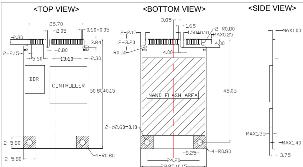
[Figure 2-1] Physical dimension
