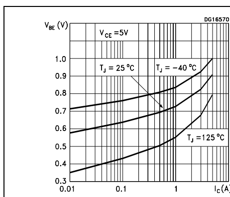
Figure 6. Base-emitter voltage
