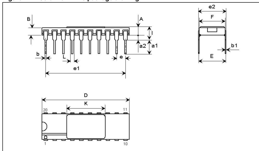
Figure 7. Ceramic DIL-20 package drawing
