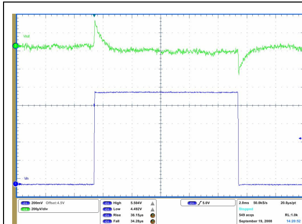
Figure 16. Line transient
