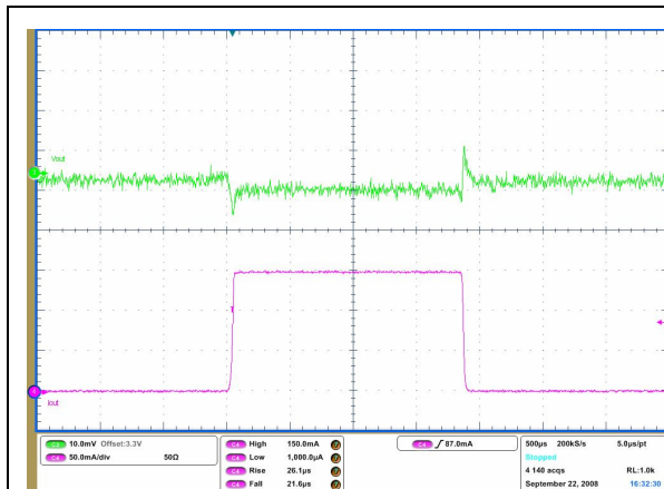
Figure 18. Load transient
