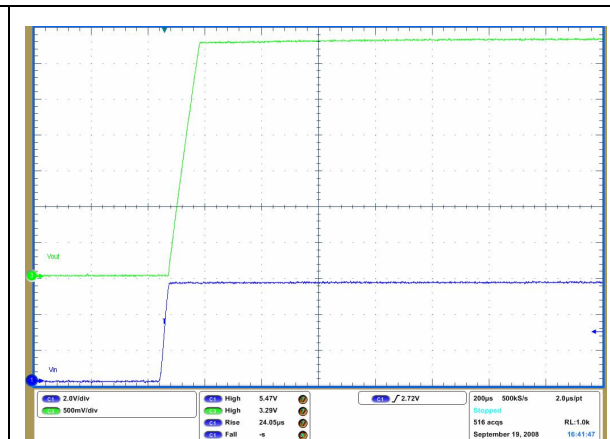
Figure 19. Startup transient
