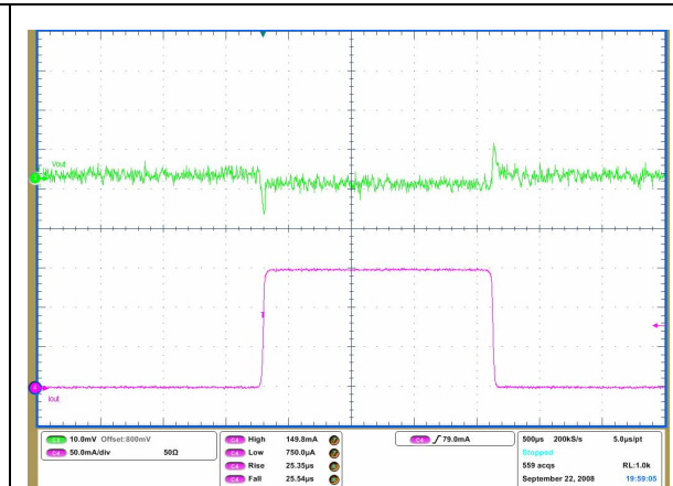
Figure 17. Load transient
