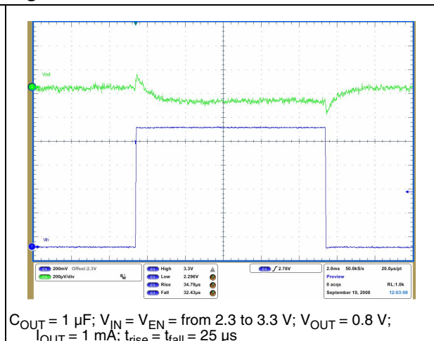
Figure 15. Line transient
