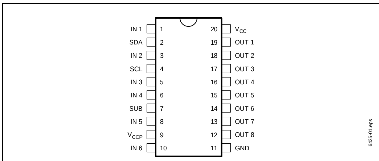
Figure 1. Pin Connections
