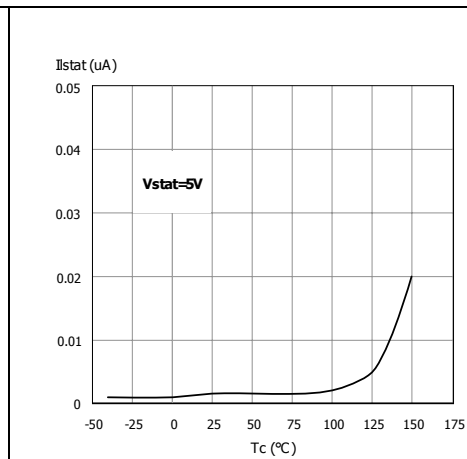
Figure 10. Status leakage current
