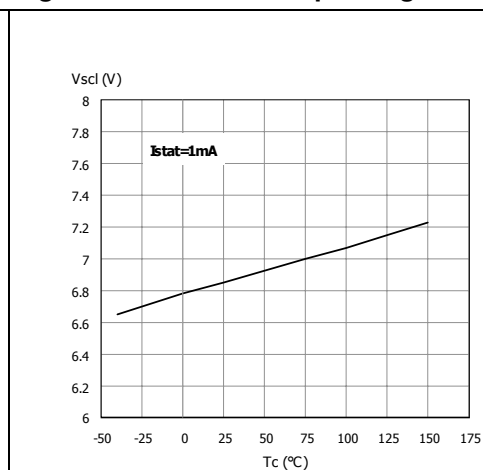
Figure 12. Status clamp voltage
