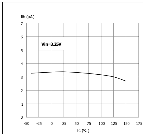
Figure 10. Status leakage current
