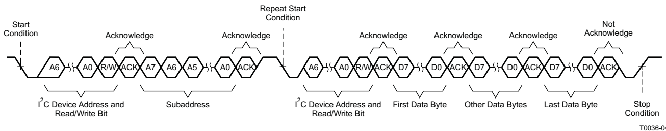
Figure 41. Multiple-Byte Read Transfer
