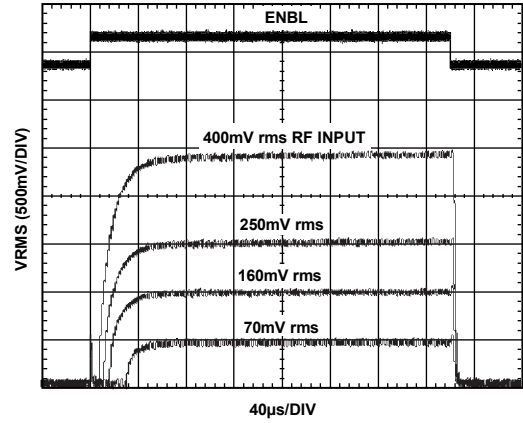
Figure 37. Output Response to Enable Gating at Various RF Input Levels, Supply = 3 V, Frequency = 900 MHz, C_{FLTR} = 1 nF, C_{OUT} = \text{Open} , R_{OUT} = \text{Open}
