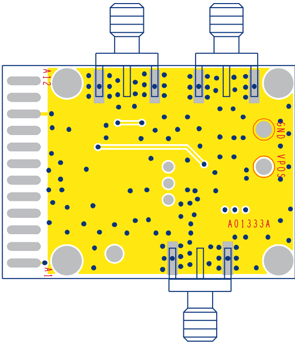
Figure 58. Layout of Evaluation Board, Circuit Side
