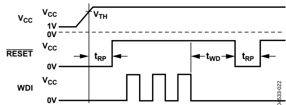
Figure 18. Watchdog Timing Diagram
