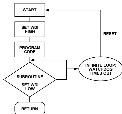
Figure 20. Watchdog Flow Diagram
